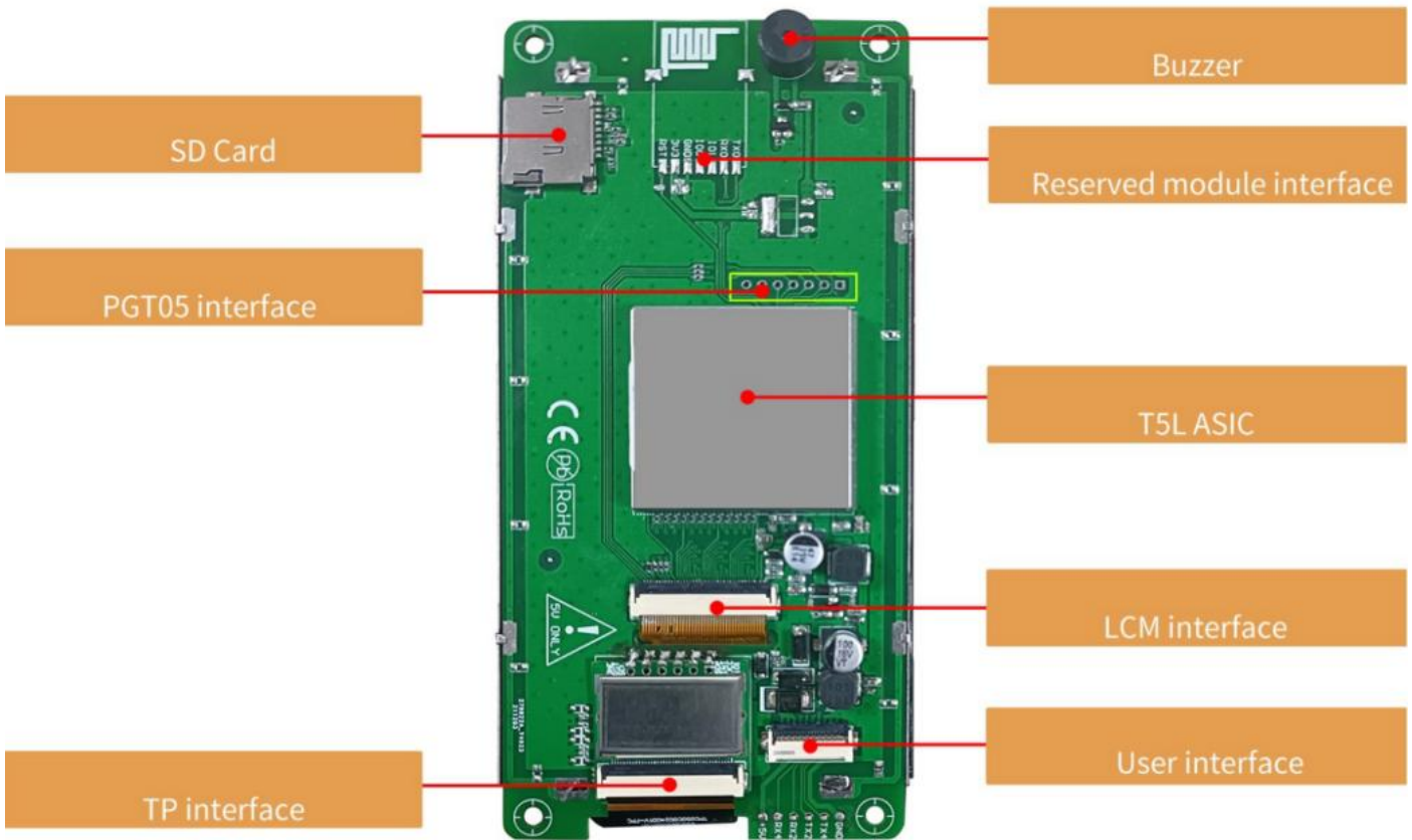
Hardware interface
