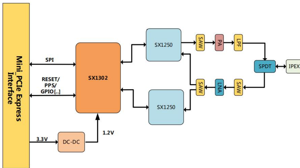
Figure 1: E106-470G27P2 function block diagram
