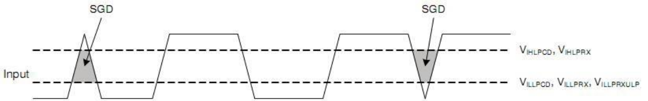
Spike/glitch rejection-DSI
