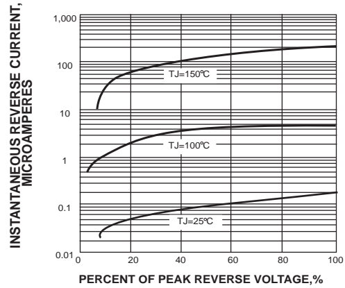
FIG. 4-TYPICAL REVERSE CHARACTERISTICS
