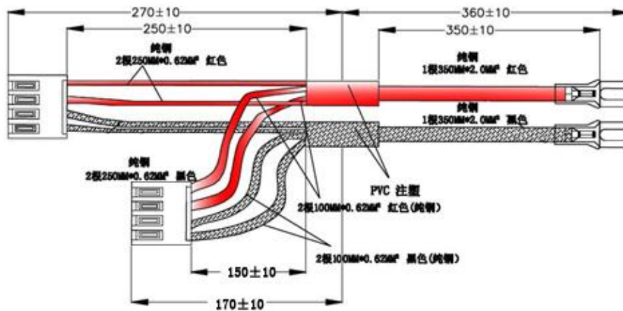
Schematic diagram of the power cord
